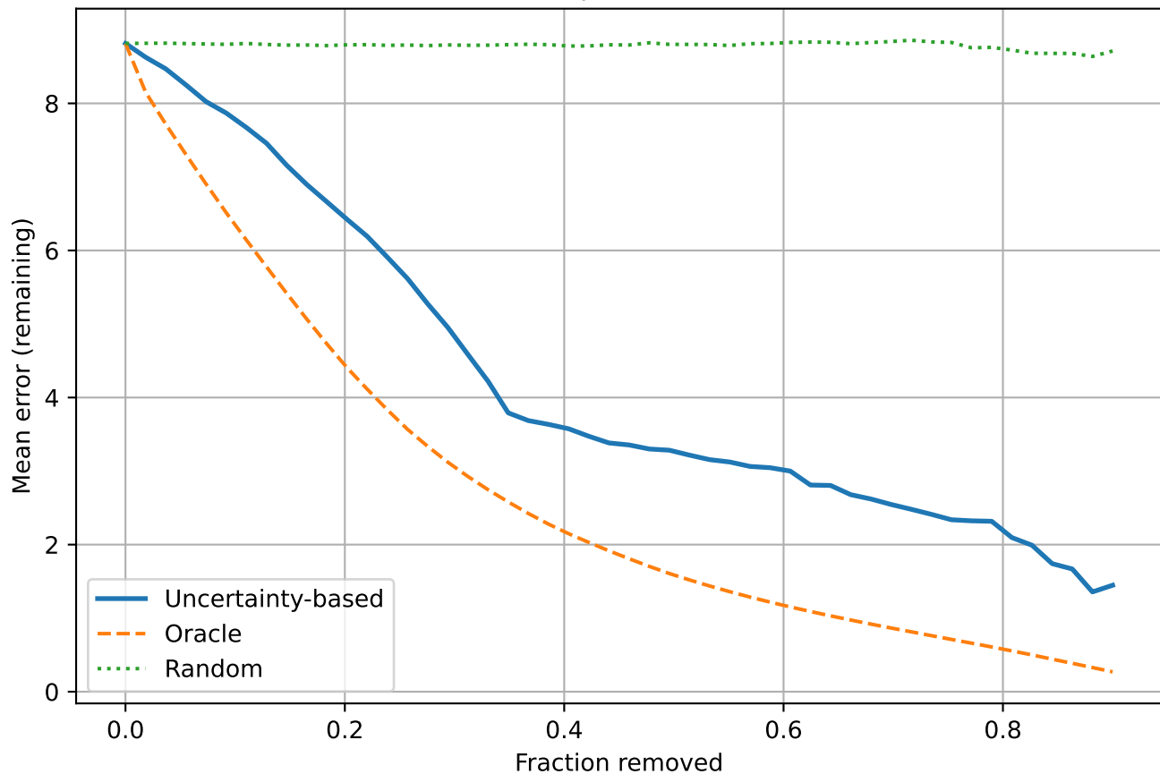
BPIC20PTC: Sparsification Curve
